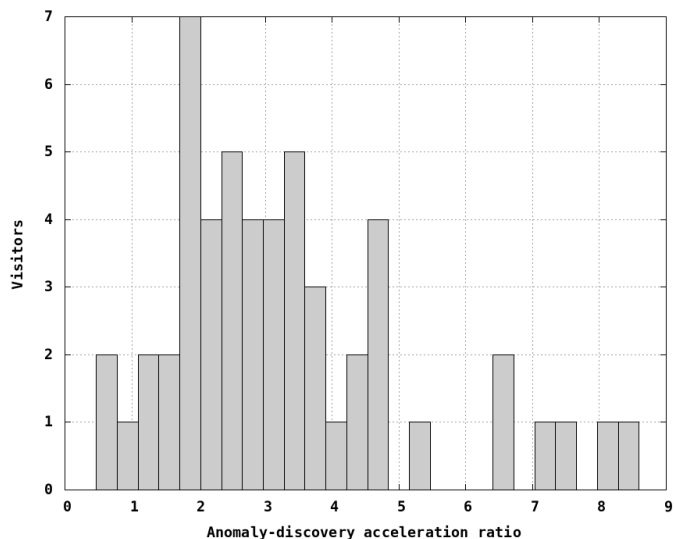
Fig. 5. Rate of discovering anomalies, as a multiple of real time, reported by visitors to the Audio Easter Egg Hunt at the Beckman Institute’s 2011 Open House. Most visitors successfully exploited the spectrogram display, finding anomalies about three times faster than real-time listening. A few visitors found anomalies over seven times faster.
